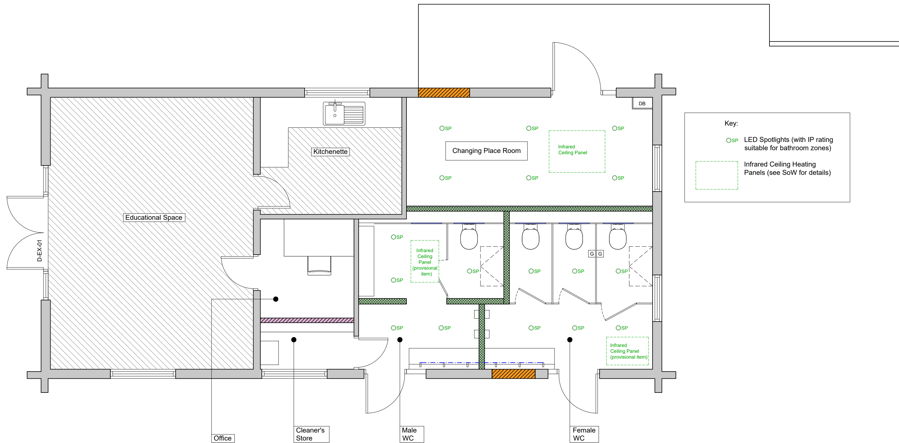
PROPOSED PLAN - CEILING 1:50
